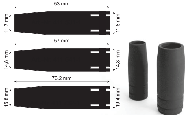
Standard Nozul
